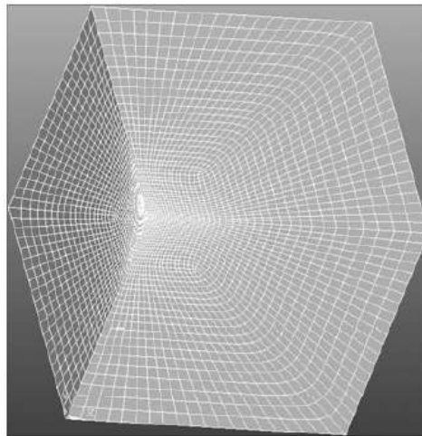
Fig 3 Three-dimensional meshed model
