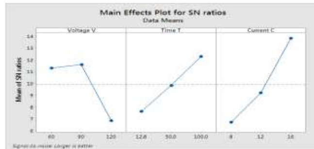
Graph 2 Individual (Main) effect plot for S/N ratio (larger-the-better) C45.Material
