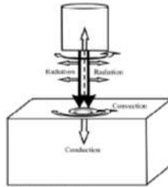
Fig. 1 Thermal model of EDM process
