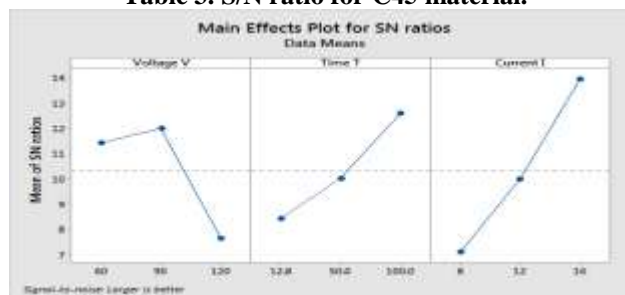
Graph 1 Individual (Main) effect plot for S/N ratio (larger-the-better) C45.Material
